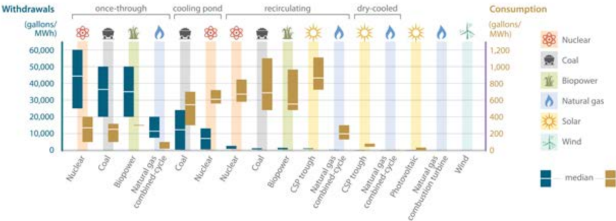
Figure 6.1. Caption from report: Water withdrawals per megawatt-hour (MWh) can range from almost zero for a solar photovoltaic, wind, or dry-cooled natural gas plant, to hundreds of gallons for an efficient plant using recirculating cooling, to tens of thousands of gallons for a nuclear or coal plant using once-through cooling. Water consumption per MWh can similarly range from almost zero for solar, wind, or gas plants using dry cooling to around 1,000 gallons (3,785 liters) for coal, oil, or concentrating solar power (CS P) with recirculating cooling. How much water a specific plant uses reflects its efficiency and age, and how much the plant is used, along with local humidity, air temperature, and water temperature (Averyt et al. 2011, MacKnick et al. 2011)
